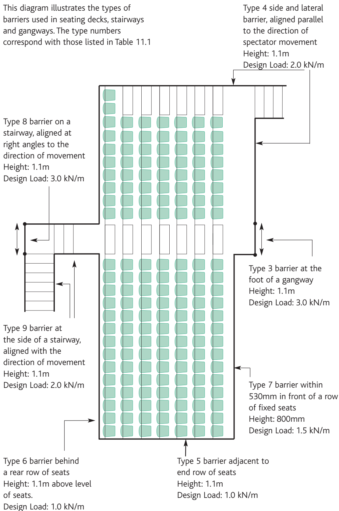
Diagram 11.1 Barrier design loads, heights and positions
