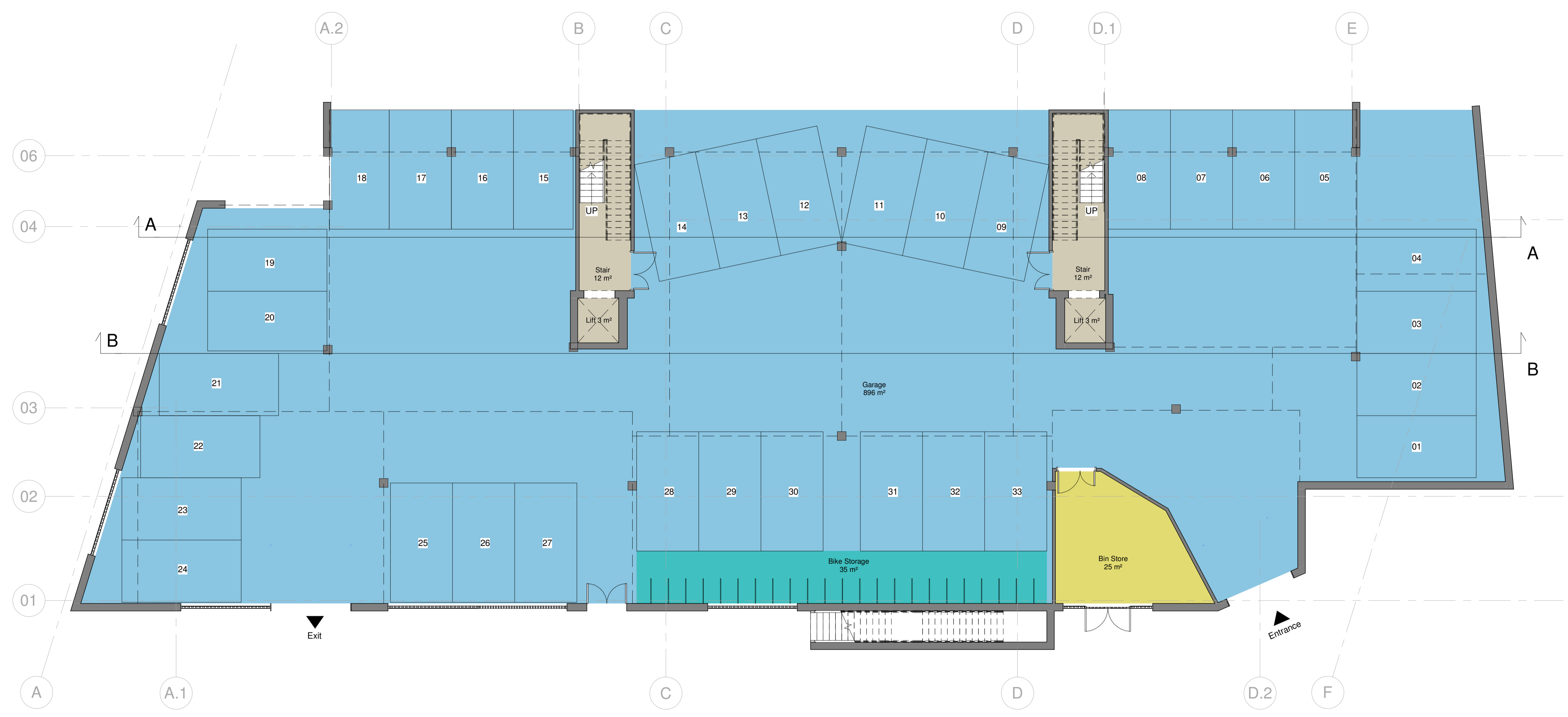
Low Ground Floor Plan 1 : 100
